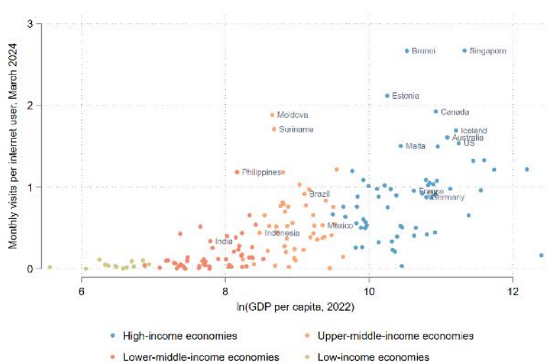
Figure 15: ChatGPT monthly visits per internet user against GDP per capita, March 2024
