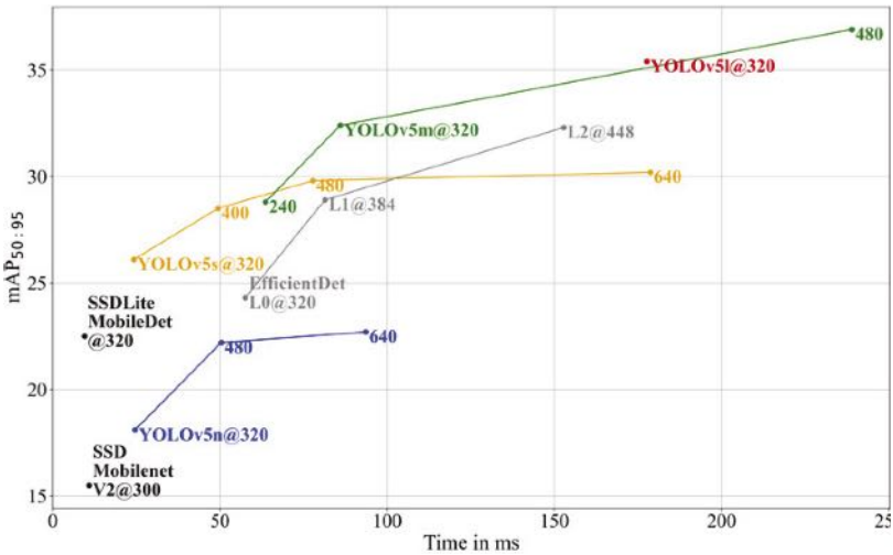
Figure 11.3 USB3 speed-accuracy comparison of different model types and configurations for edge TPU deployment.
