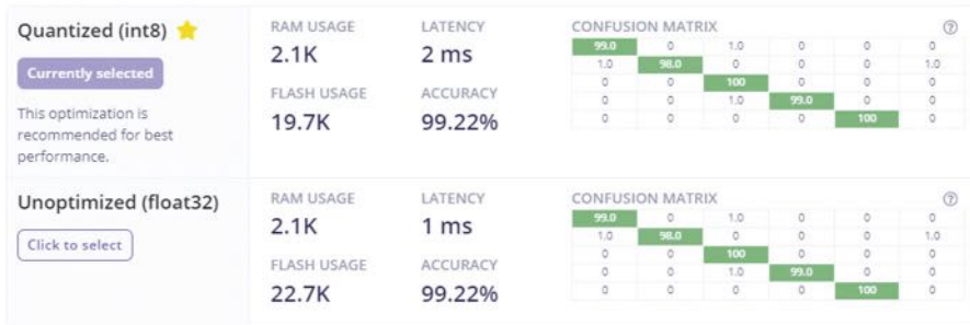
Figure 12.7 A comparison between int8 quantized and unoptimized versions of the same model, showing the difference in performance and results.
