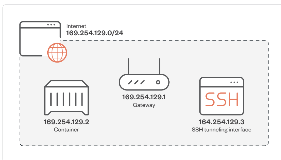
Figure 10. Default network scheme
