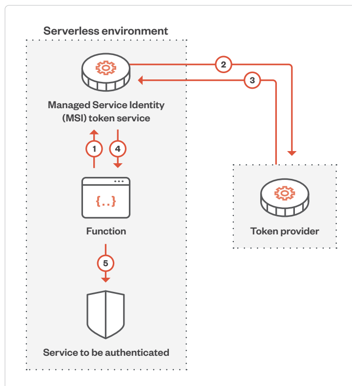
Figure 26. The architecture of a serverless IDP service
