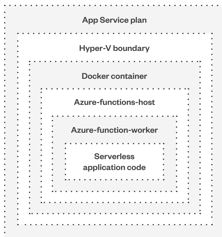
Figure 33. Azure App Service plan inclusions
