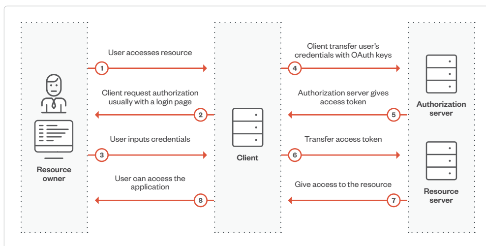
Figure 53. An ideal token management service
