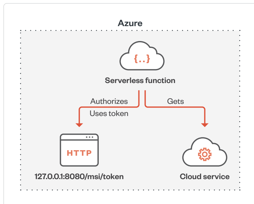
Figure 23. An example of how a system-assigned managed identity is used
