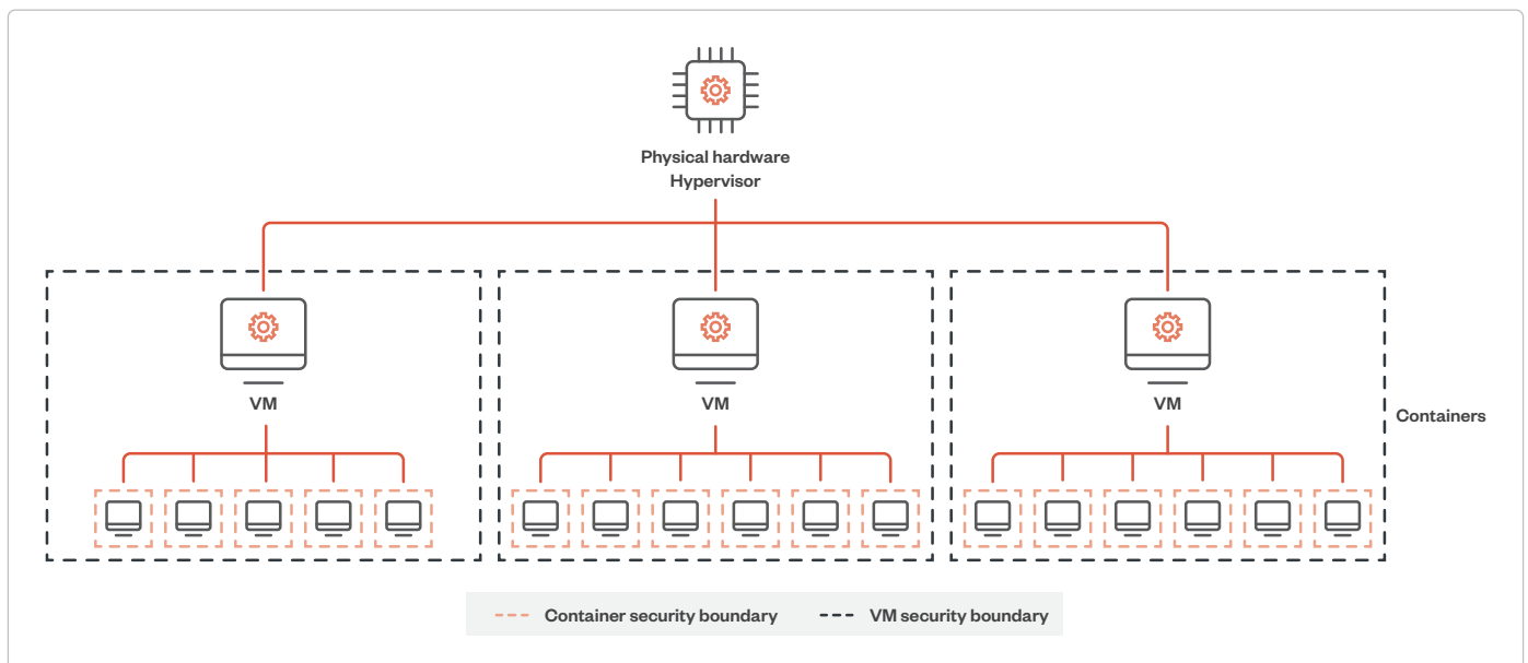
Figure 1. Container security and VM security boundaries
