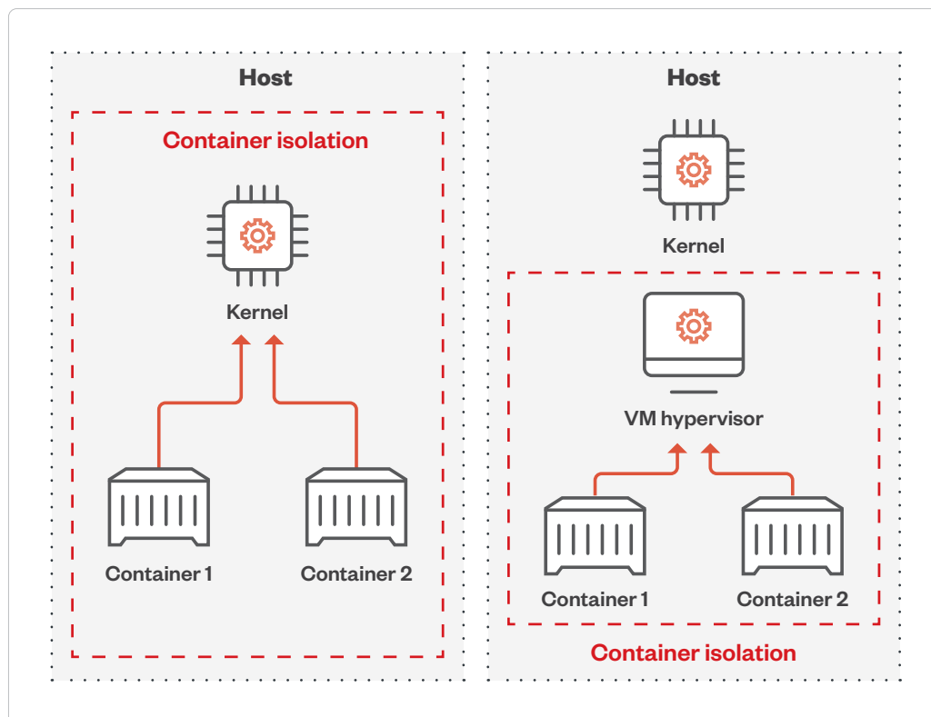
Figure 2. A comparison of standard containers and micro VM-based containers
