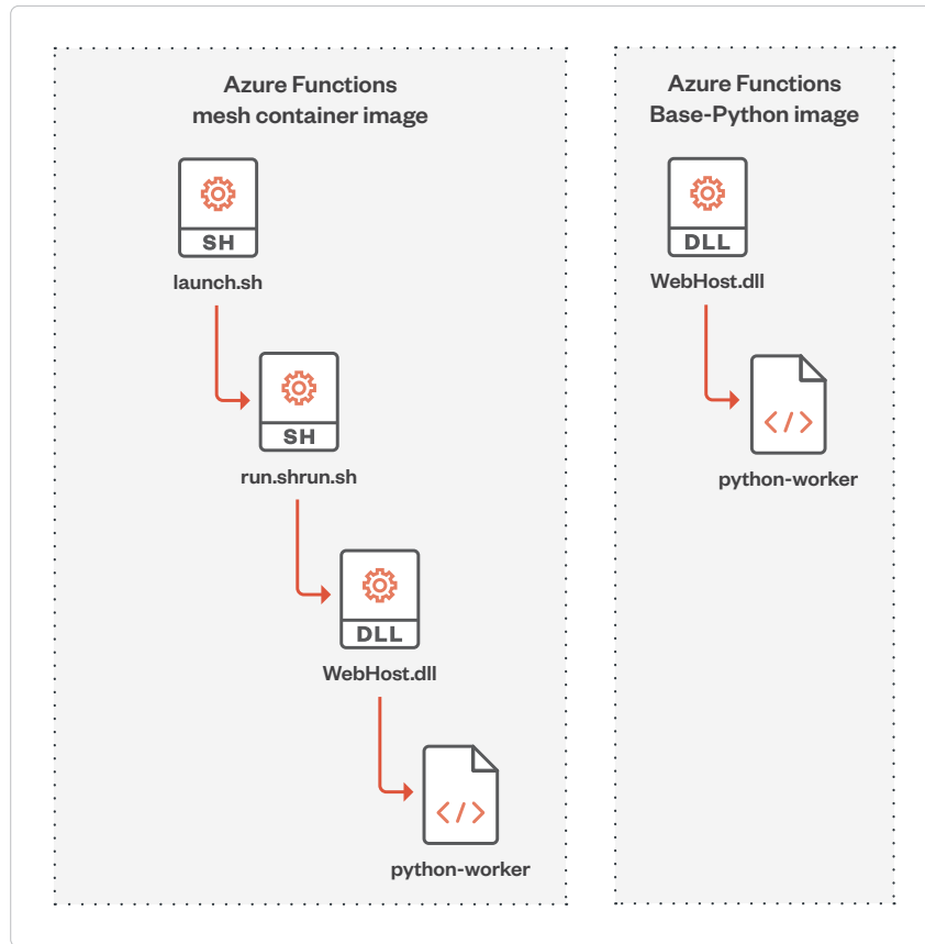
Figure 37. Comparison of container images
