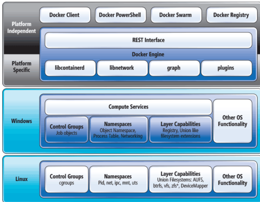
Figure 3. Host platform implementation details of Windows and Linux
