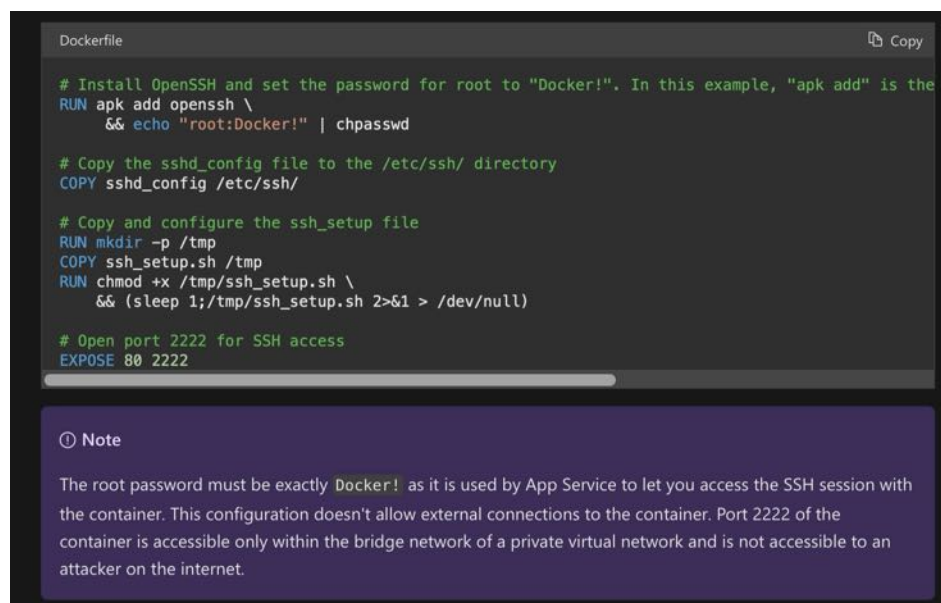
Figure 8. Screenshot of a custom container tutorial from Azure
