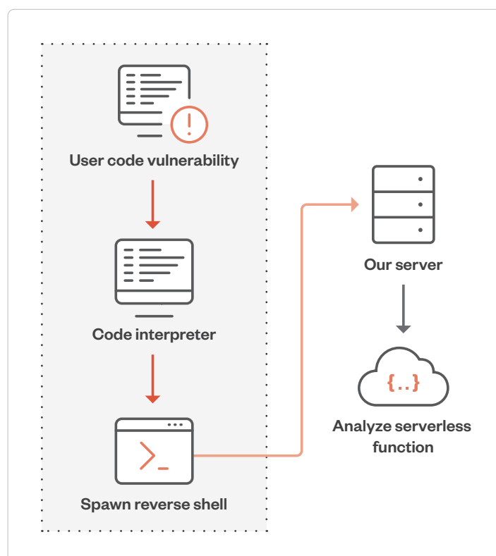
Figure 4. Attack simulation of a serverless function
