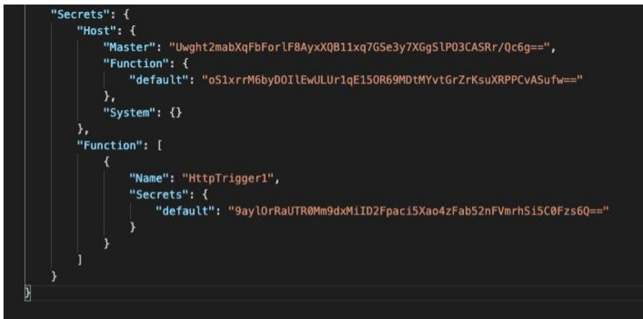
Figure 22. Leaked secrets from decrypted context
