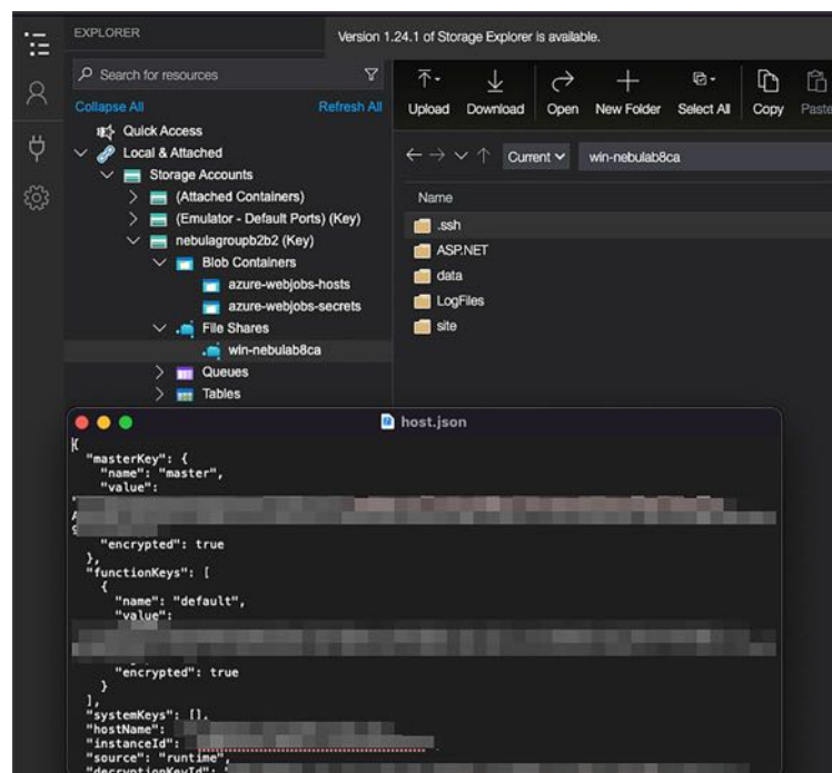
Figure 32. Connection to Azure Storage using an environmental variable connection string
