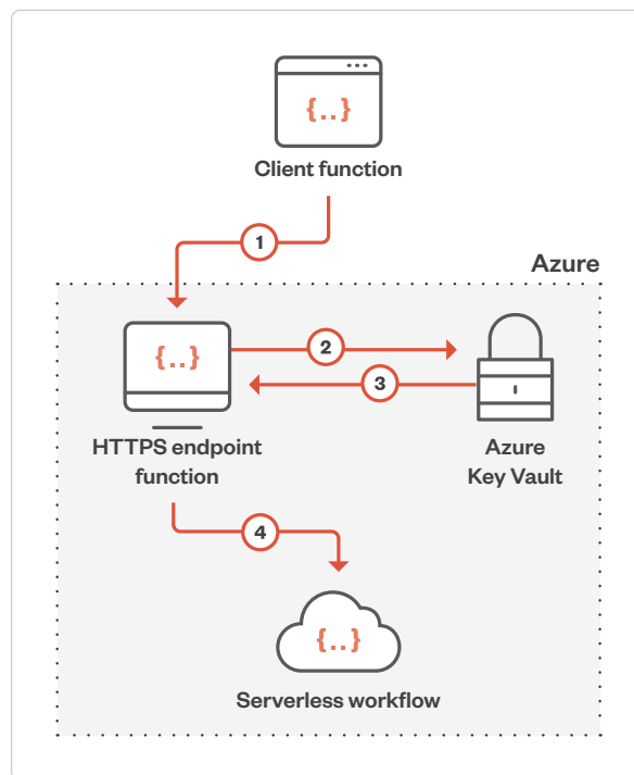
Figure 16. Azure authentication approaches
