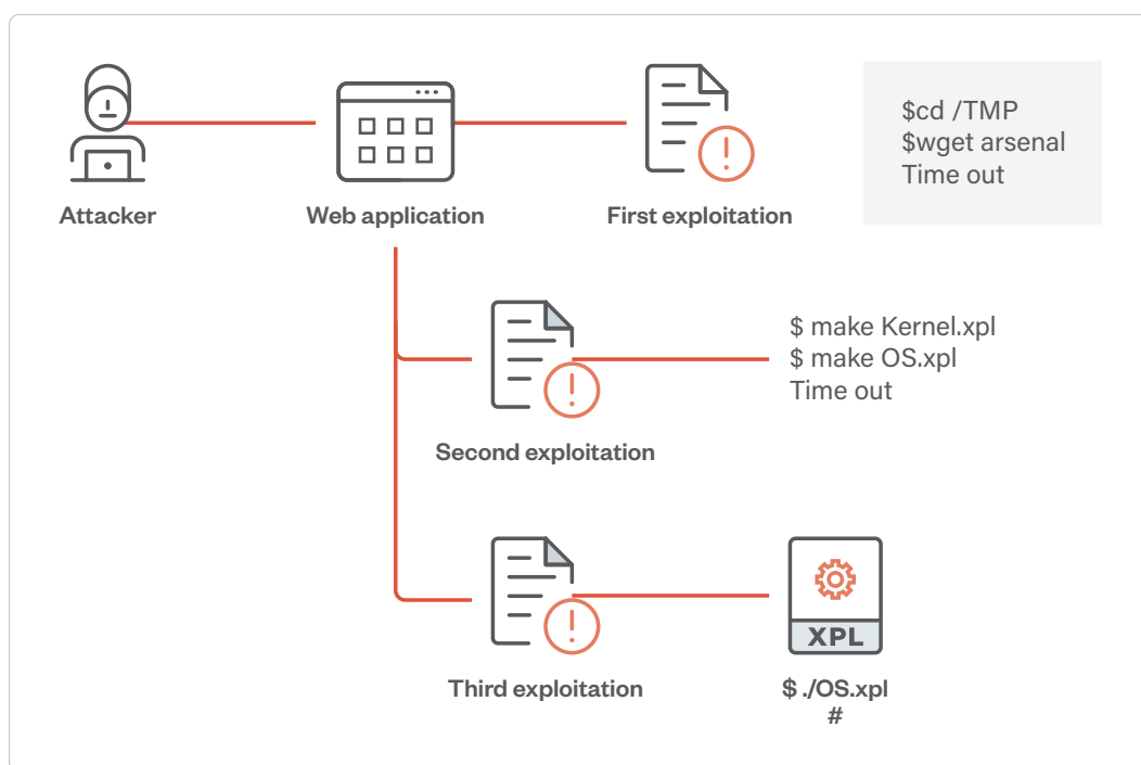
Figure 52. An example of an exploitation wherein an attacker breaks as a non-root user and downloads its arsenal under “/tmp”; the attacker then uses native building tools to compile exploits for further exploitation
