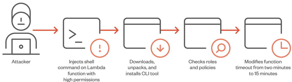
Figure 57. An AWS Lambda kill chain for a function with high permissions
