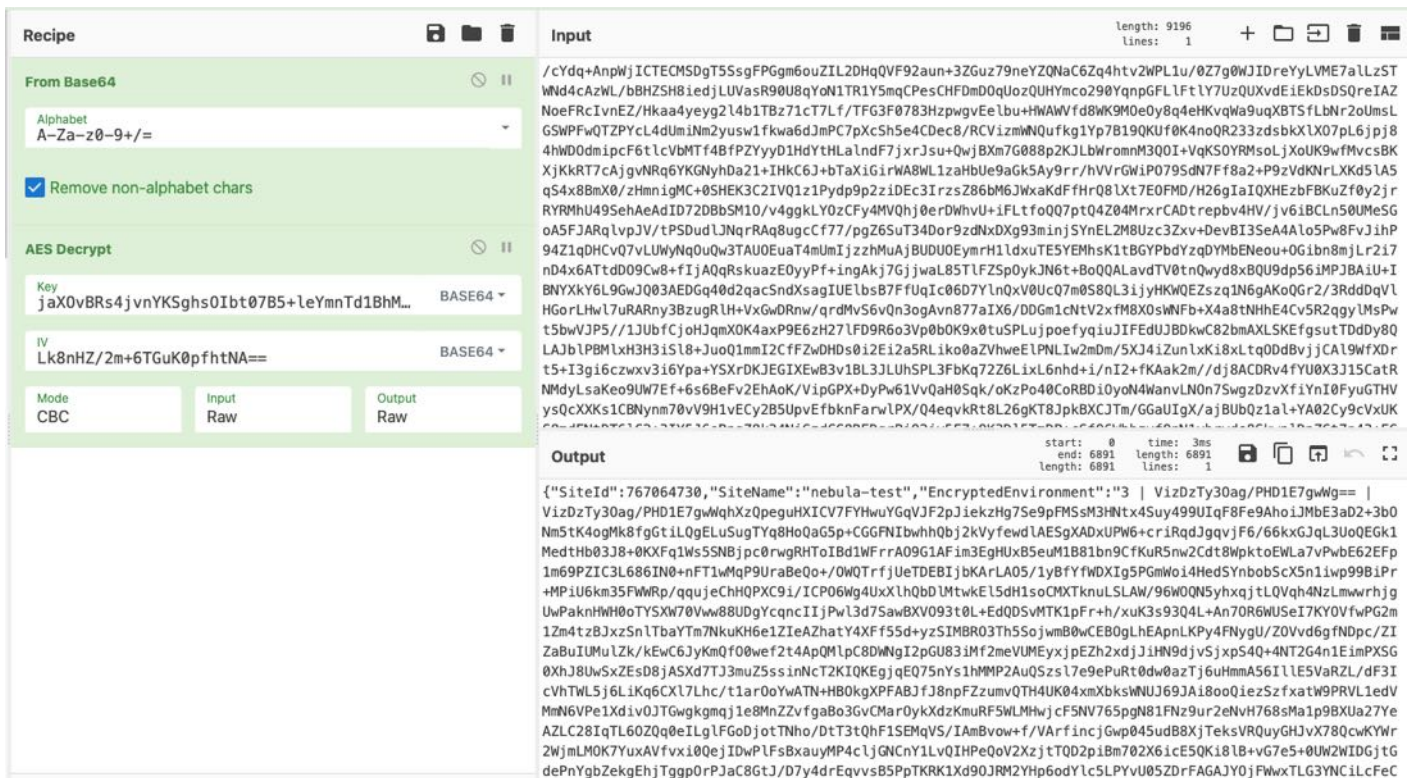
Figure 21. Decrypted container context
