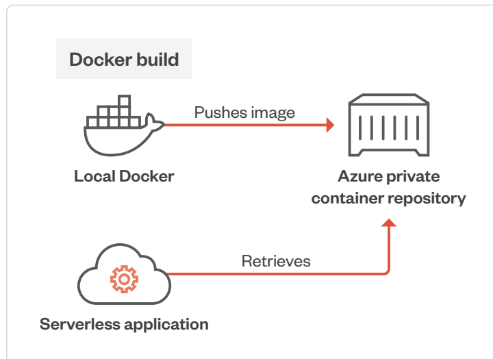
Figure 36. Deployment diagram
