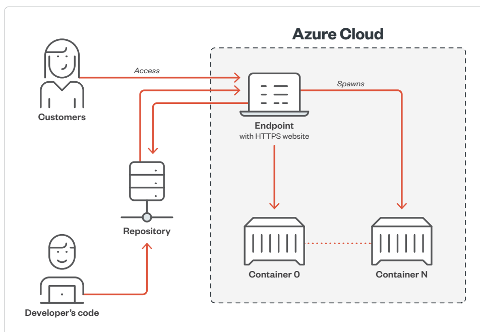
Figure 6. Azure App Service with CI/CD integration
