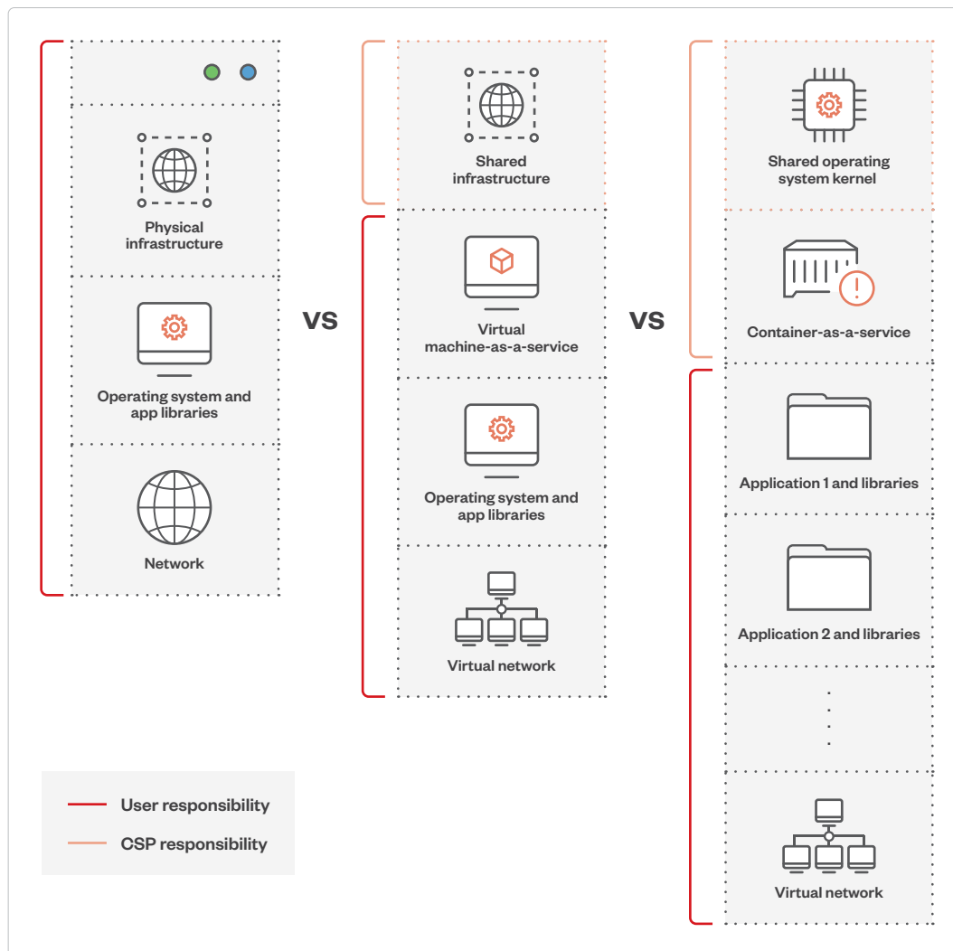
Figure 48. The shared responsibility shift over different infrastructures
