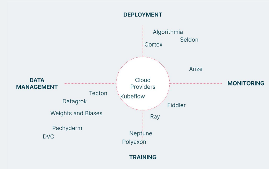
Figure 8: MLOps software with poles of specialization in lifecycle stages and all-in-one platforms gravitating towards poles (or middle if no particular pole)
